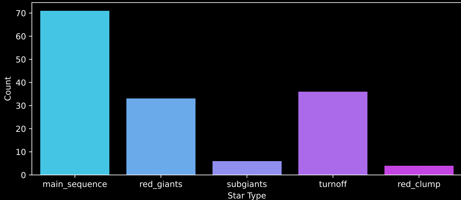
APOGEE DR17 Field: [041+48_MGA] Count plot of Star Type
