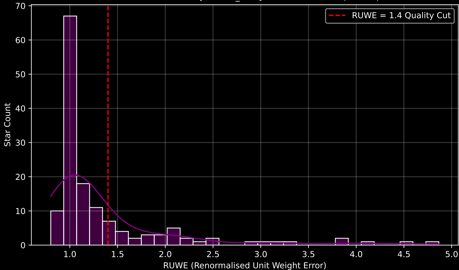
GAPOGEE DR17 Field [041+48_MGA] RUWE Distribution (n= 144)
