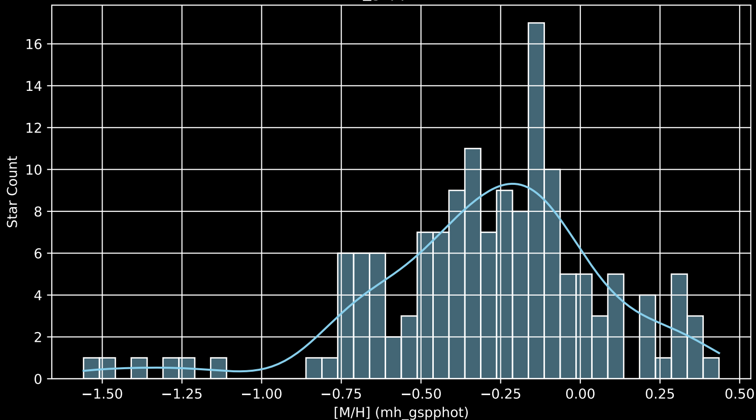
APOGEE DR17 Field: [041+48_MGA [M/H] (mh_gspphot) (n= 148)
