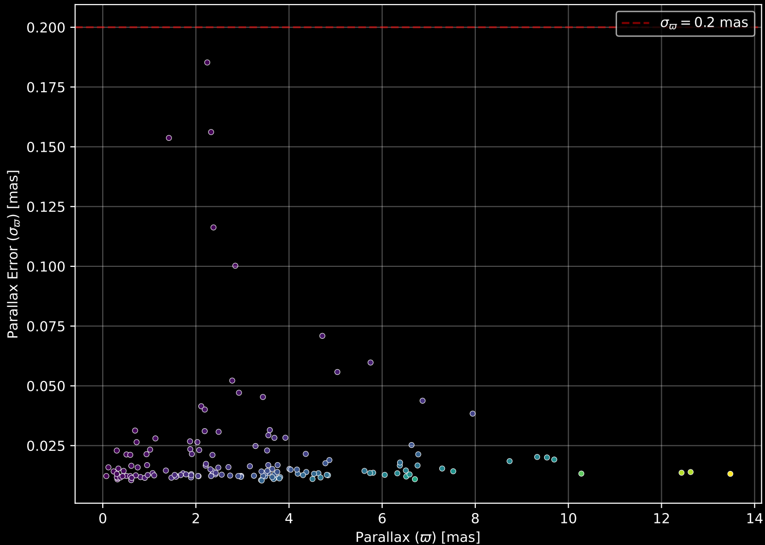
APOGEE DR17 Field: [041+48_MGA] Parallax Quality (n= 150)
