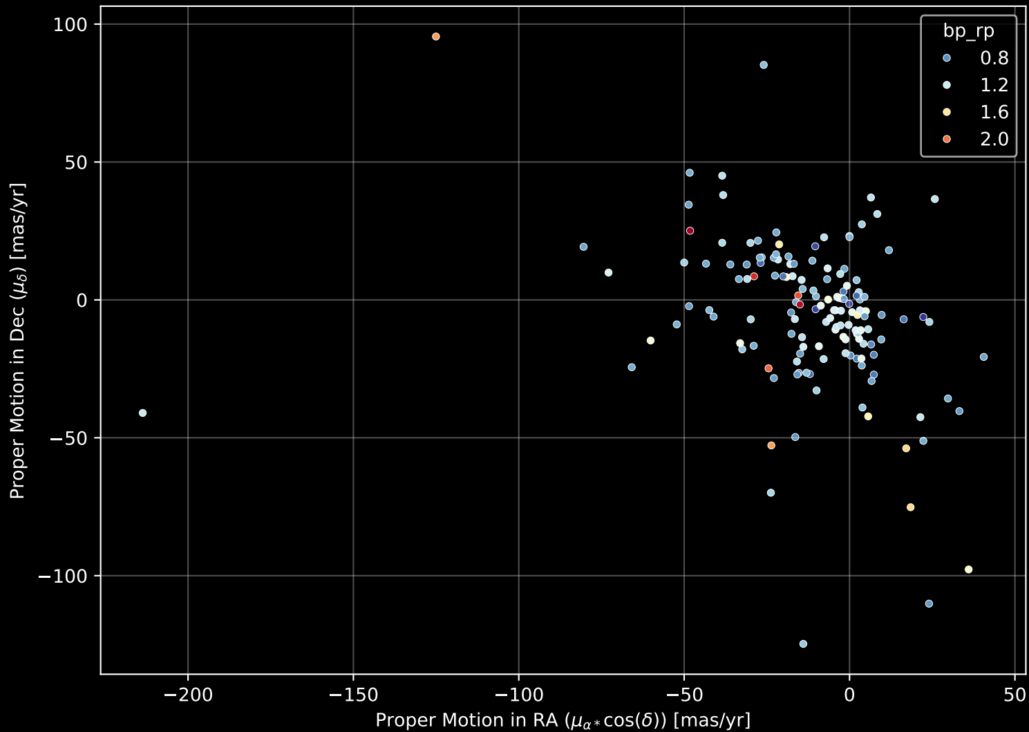
APOGEE DR17 Field: [041+48_MGA] Proper Motion Diagram (n= 150)
