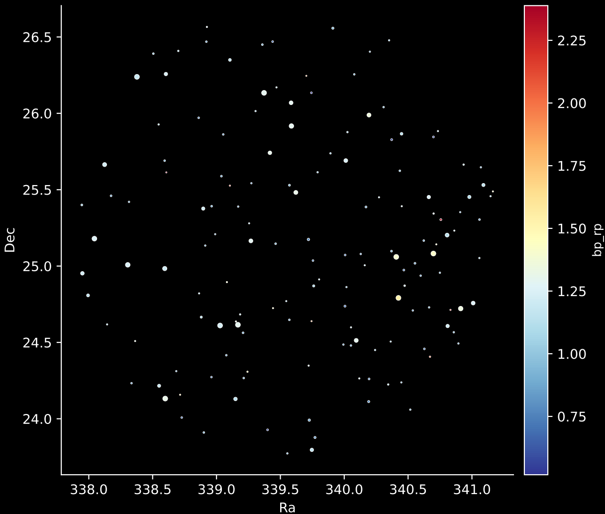
APOGEE DR17 Field: [041+48_MGA] Stars: 150
